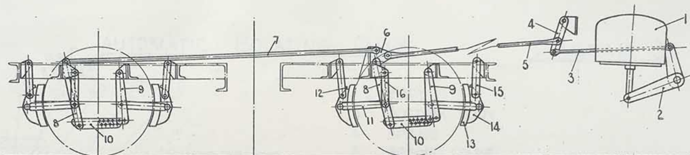
BRAKEWORK ON TRAILER BOGIE. BIRMINGHAM DIESELS
