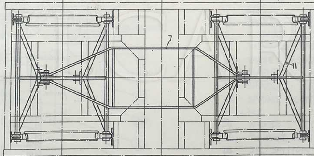
BRAKEWORK ON TRAILER BOGIE. BIRMINGHAM DIESELS
