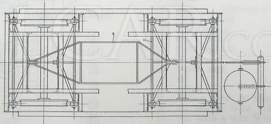
BRAKEWORK ON TRAILER BOGIE CRAVEN BUILT DIESELS.
