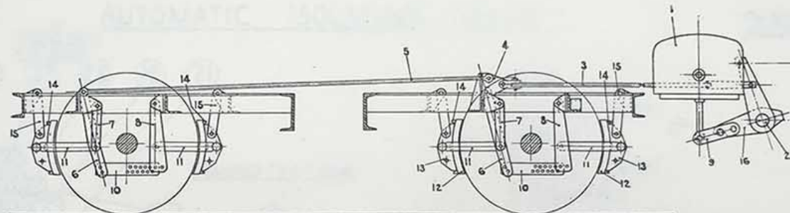
BRAKEWORK ON TRAILER BOGIE CRAVEN BUILT DIESELS.
