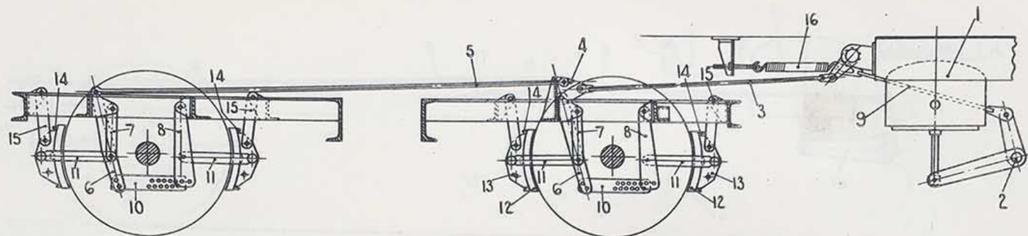
BRAKEWORK ON TRAILER BOGIE. GLOUCESTER BUILT DIESELS.
