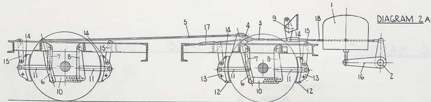
BRAKEWORK ON TRAILER BOGIE. PARK ROYAL DERBY GLOUCESTER STEEL BUILT DIESELS.
