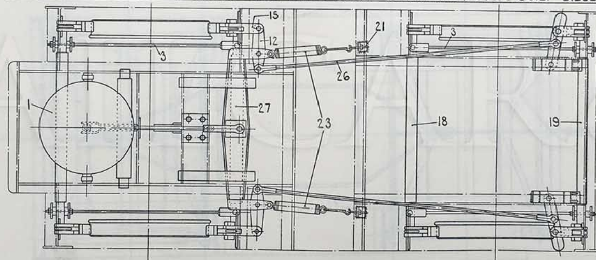
BRAKEWORK ON DRIVING BOGIE. PARK ROYAL DERBY GLOUCESTER STEEL BUILT DIESELS
