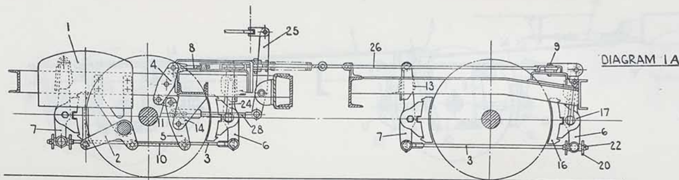
BRAKEWORK ON DRIVING BOGIE. PARK ROYAL DERBY GLOUCESTER STEEL BUILT DIESELS
