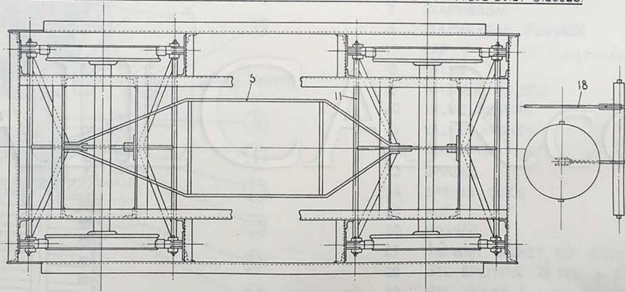
BRAKEWORK ON TRAILER BOGIE. PARK ROYAL DERBY GLOUCESTER STEEL BUILT DIESELS.
