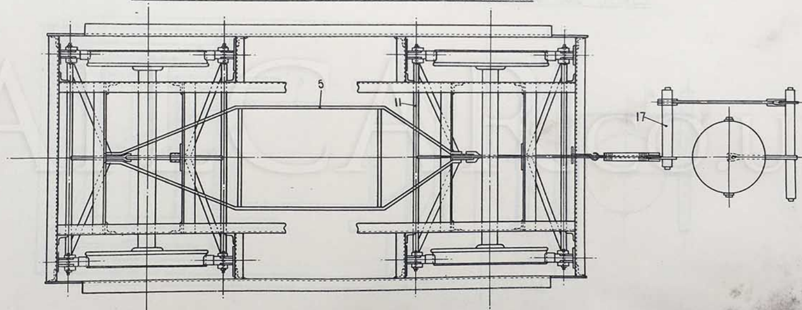
BRAKEWORK ON TRAILER BOGIE. GLOUCESTER BUILT DIESELS.
